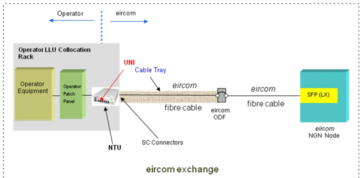
Figure 5 WSEA In-Building Handover
