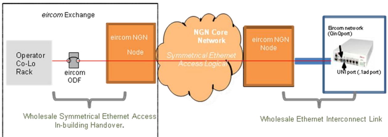
Figure 7: Wholesale Symmetrical Ethernet Access In-building Handover - logical
